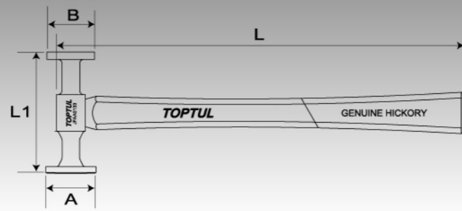
■ Standard Bumping Hammer - Crowned Face
