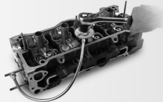
Loosening & tightening the screw to zero the gauge
