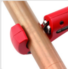
Retractable reamer
