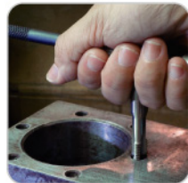
2. Tap re-drilled hole using tap
