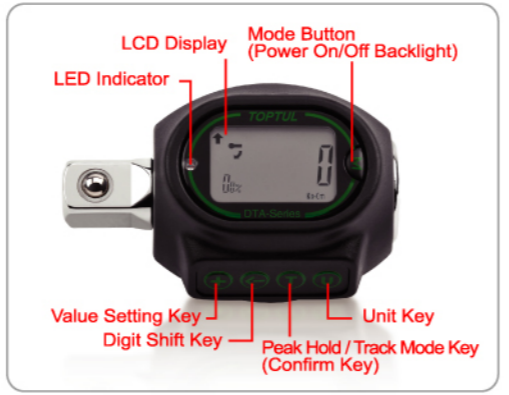
■ Rotatable mechanism design can reach total 240° view area for easily reading the torque value on the LCD display.
