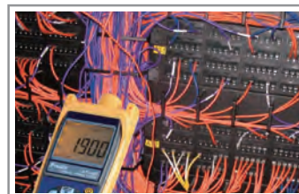
End-to-end loss test by MT-7600
