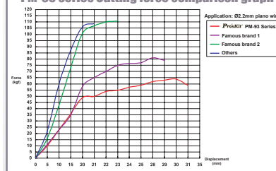
PM-93 series Cutting force comparison graph
