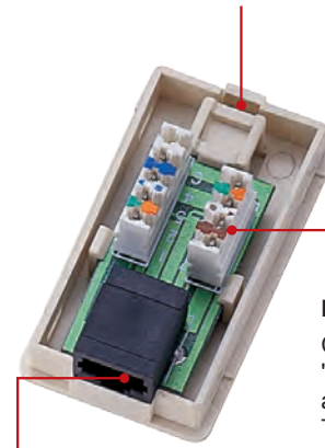
Unshielded RJ45 jack
